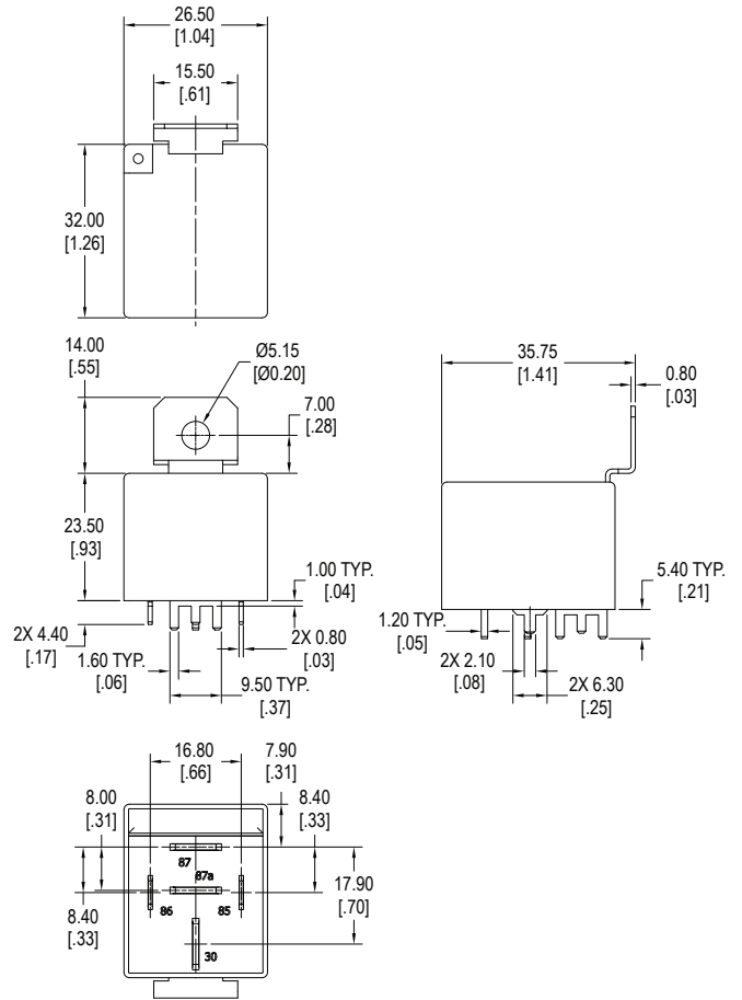
1C Metal Bracket, PC Terminals
