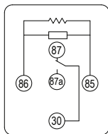
1C with Resistor
