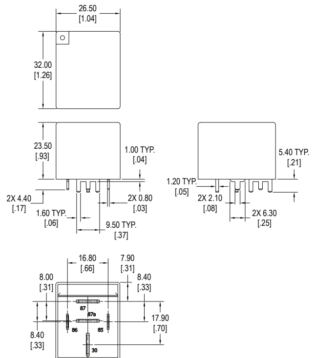
1C Standard, PC Terminals
