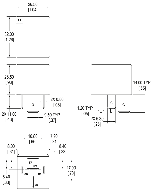
1C Standard, Quick Connect
