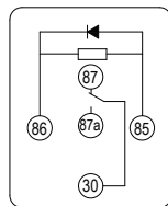
1C with Diode
