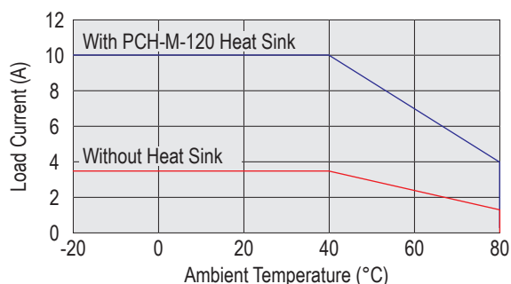
Max Load Current vs. Ambient Temperature (10A, 400V)
