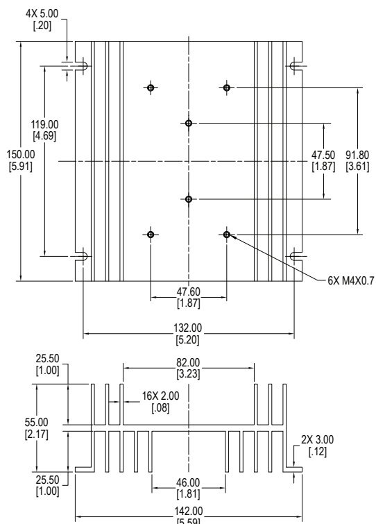
PCH-H-150 Heat Sink
