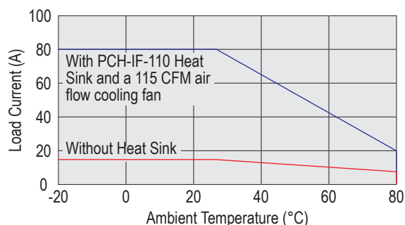
Max Load Current vs. Ambient Temperature (80A, 100V)
