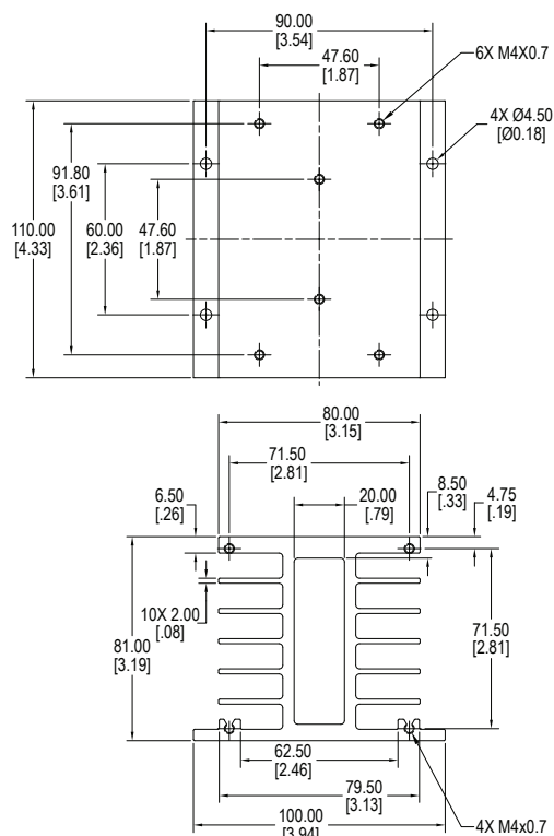
PCH-IF-110 Heat Sink
