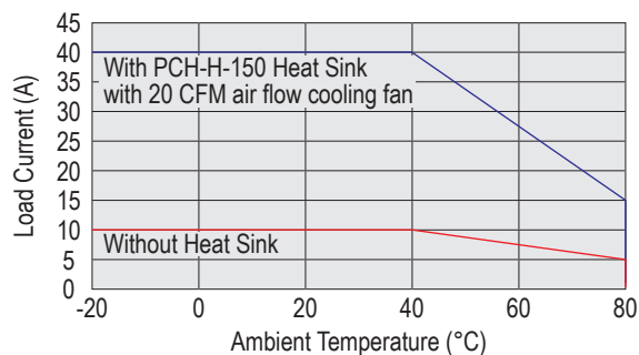
Max Load Current vs. Ambient Temperature (40A, 50V)
