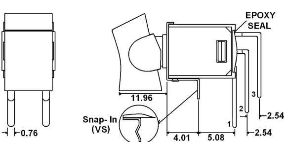
V (VS - Snap In) = Vertical mount, right angle PC pins, double pole
