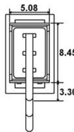
H (HS - Snap In) = Horizontal mount, right angle PC pins, double pole
