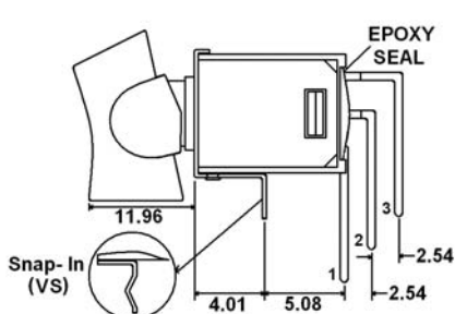
V (VS - Snap In) = Vertical mount, right angle PC pins, double pole
