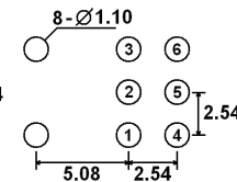
H (HS - Snap In) = Horizontal mount, right angle PC pins, double pole
