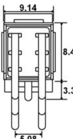
V (VS - Snap In) = Vertical mount, right angle PC pins, double pole
