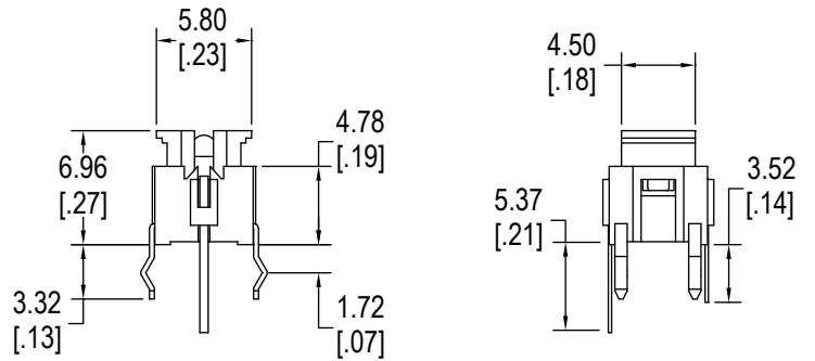
CL1200 for Cap C, D, E & F
