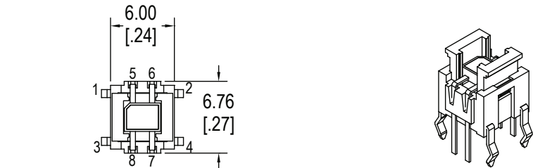
CL1200 for Cap A, A1, B & B1
