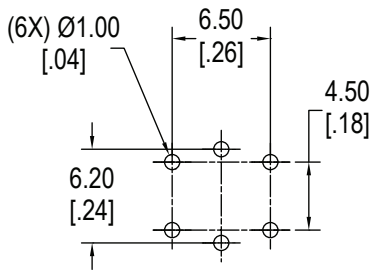
Thru Hole
