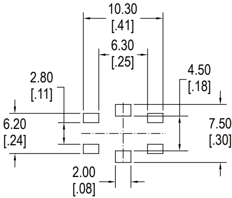
Surface Mount
