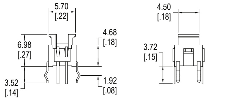
CL1200 for Cap A1, C, D, E & F with RGB LED
