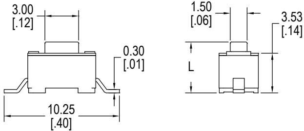
Gull Wing
