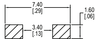
J Lead
