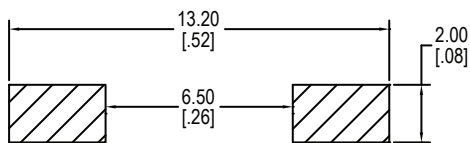
Gull Wing
