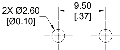
Panel Mounting
