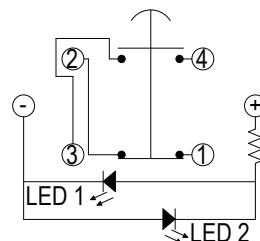
SPST NO + SPST NC, Dual Color LED
