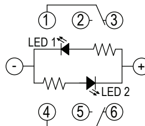
Double Pole Double Throw
