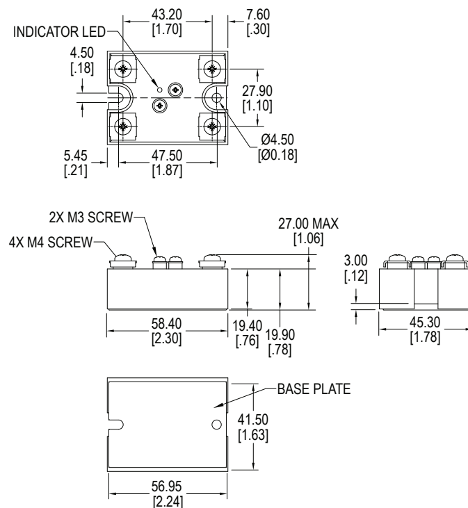
1SS, Input Control for Dual Output, Screw Terminal Input/Output, with LED Indicator
