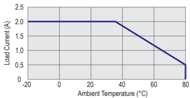
Max Load Current vs. Ambient Temperature
