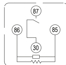
1A with Resistor
