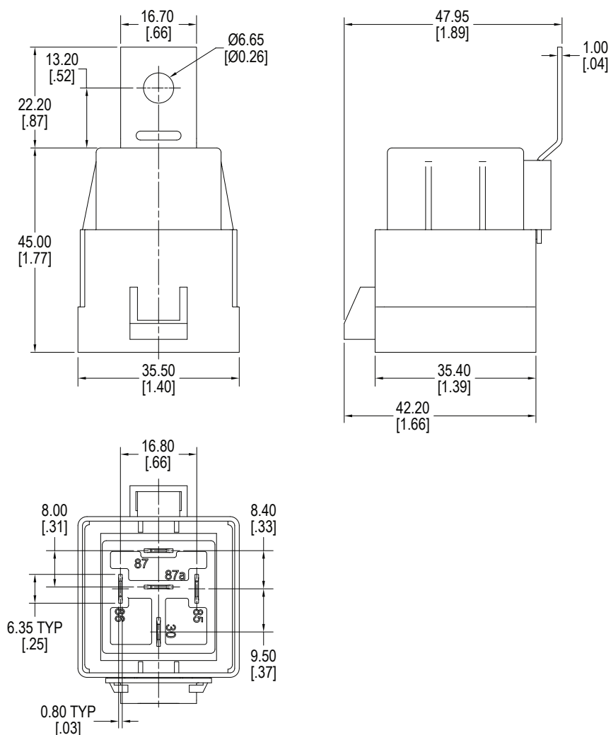
A2S, Quick Connect, Sealed
