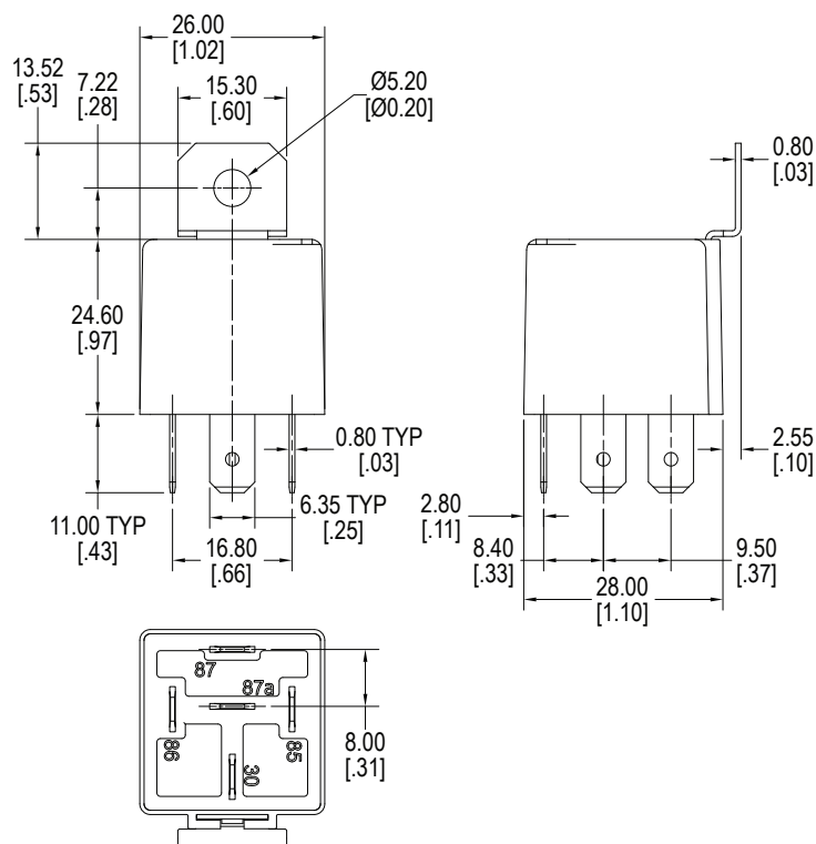
A2M with Quick Connect, Sealed
