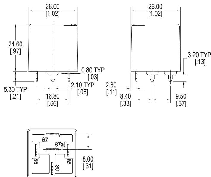
A2 with PC Pins, Sealed
