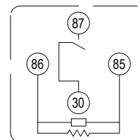
1A with Resistor
