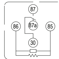
1C with Resistor
