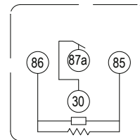
1B with Resistor
