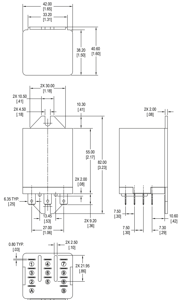
C1 - Side Flange
