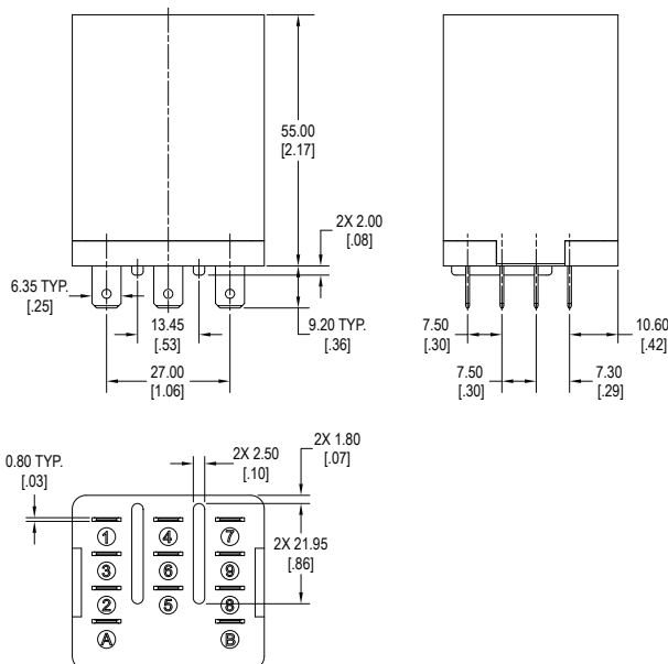
C - Plain Case
