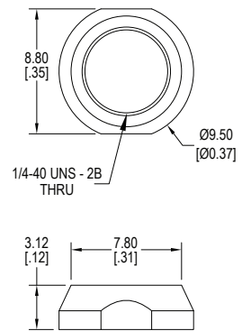
Locking Ring
