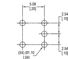
C DPDT
