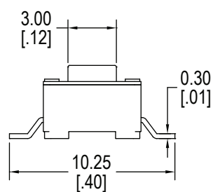
Gull Wing
