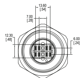
Double Pole Bottom View
