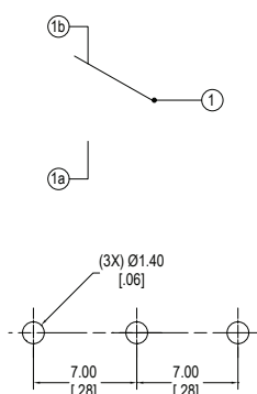
Single Pole Double Throw
