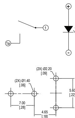
Single Pole Single Throw with LED
